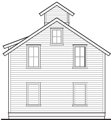
Left Elevation
